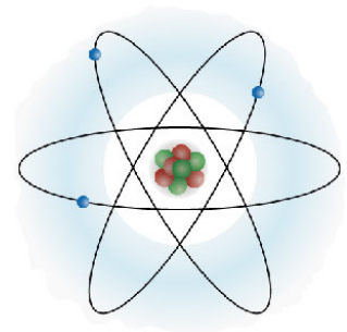
Classic model of the atom.
