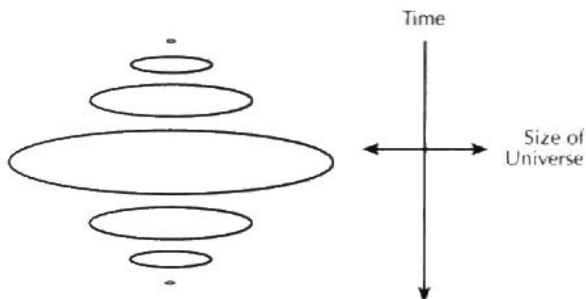
Figure 2. Time and size in a closed relativistic universe.
