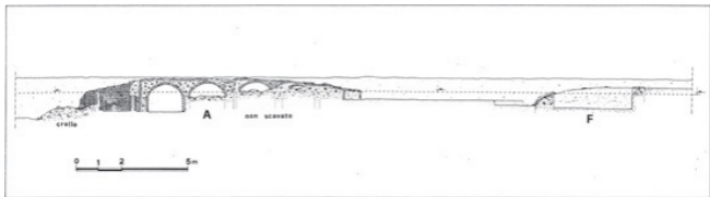
Figure 13.3. Cumae (Campaniae). Section of the Isaeum: A. podium ; F. pool.
