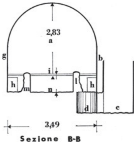
Figure 16.2b. Transverse (B-B) section. The fascia walls of the Phase IIIa-b podia are marked m and l.
