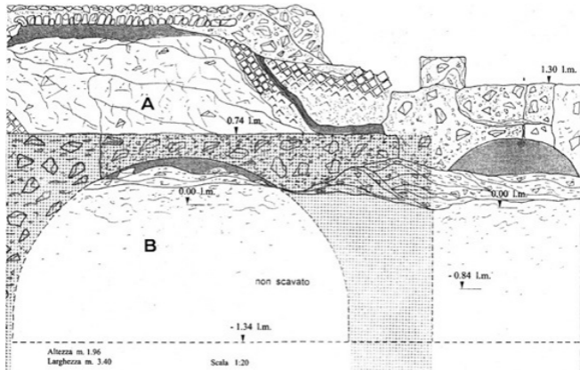
Figure 13.4. Cumae (Campaniae). Section of the Isaeum: A. upper podium ; B. lower structure.
